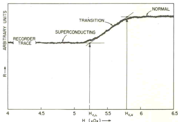
Fig. 1. A typical recorder trace showing resistance versus applied magnetic field and the method of determining H_{c,u} and H_{c,l} . This trace was taken at 4.2°K and approximately 37 kilobar.
